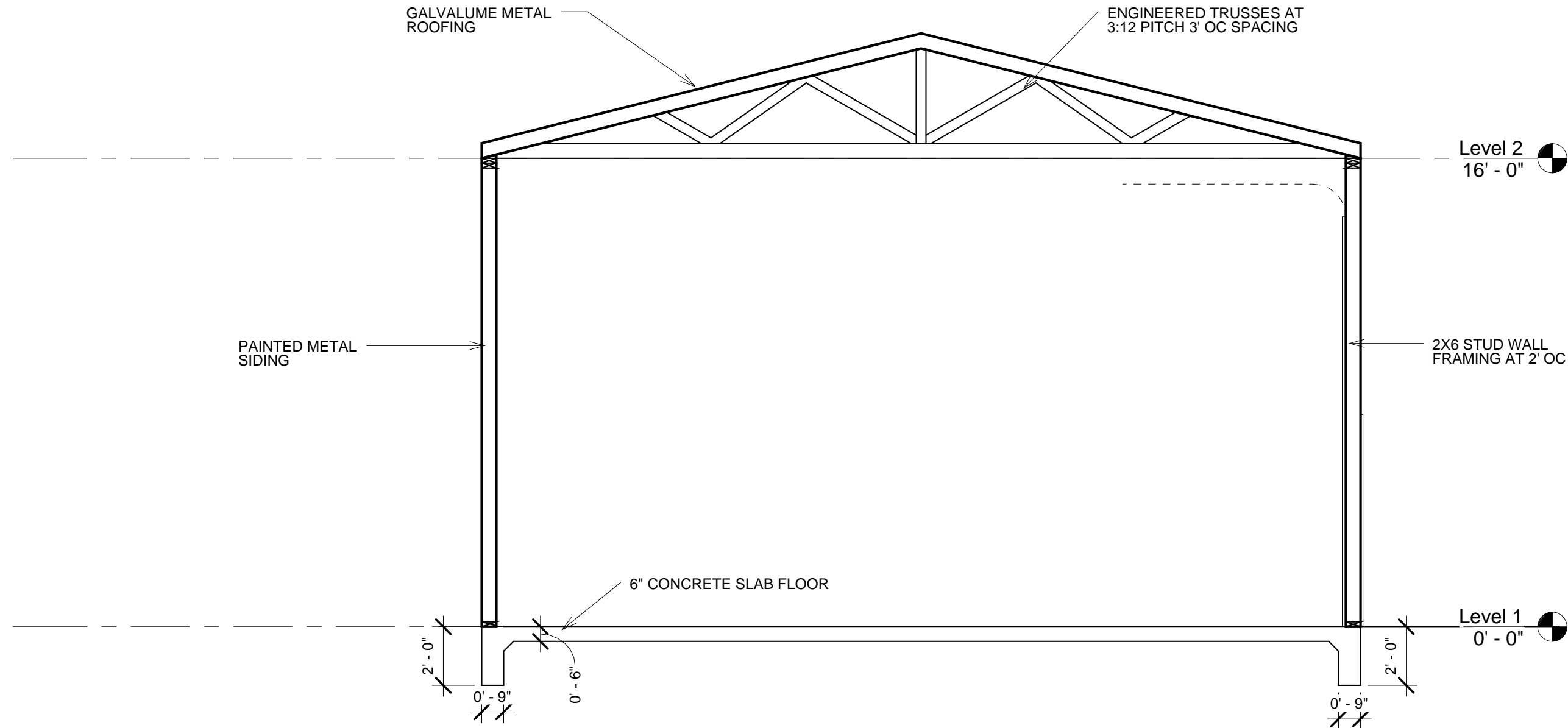
1 Section 1 1/4" = 1'-0"
