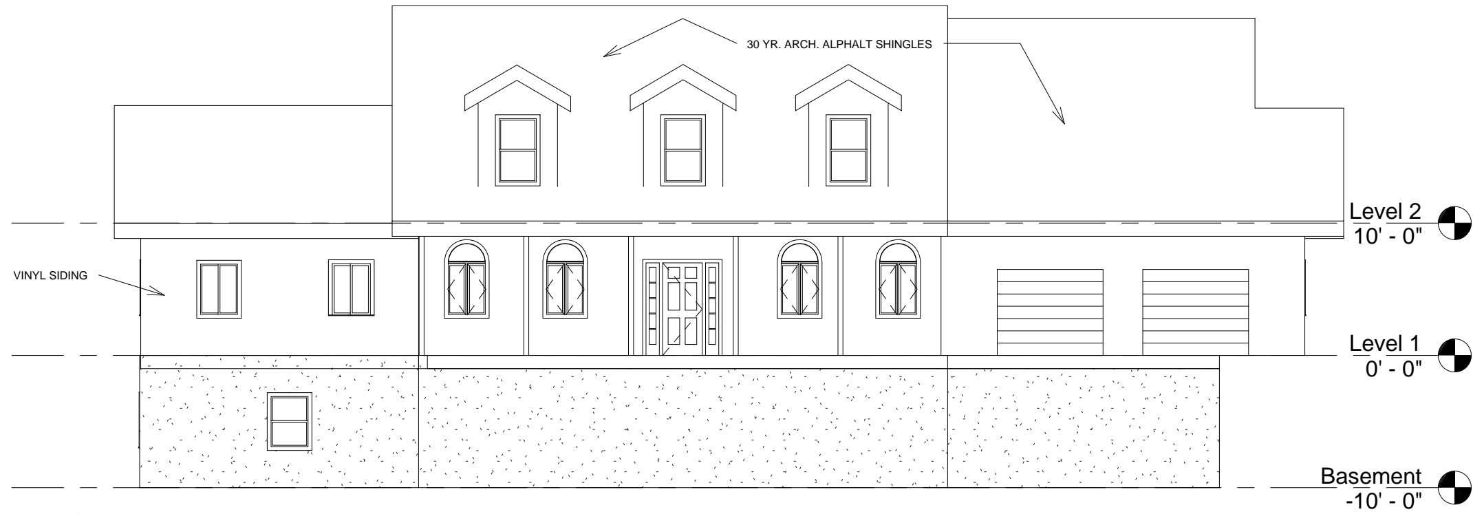
① South 1" = 10'-0"
